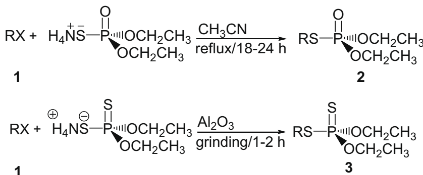
Scheme 1. Synthesis of phosphorothioates and phosphorodithioates.
